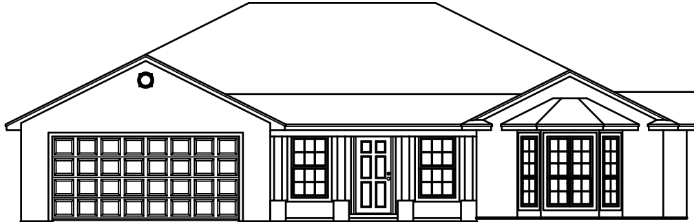
Front Elevation
